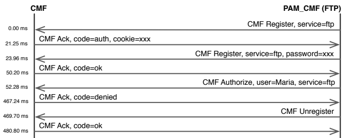
Figure 4 - Messages related to service registration and user verification, with unsuccessful authorization, captured by a monitoring application.
