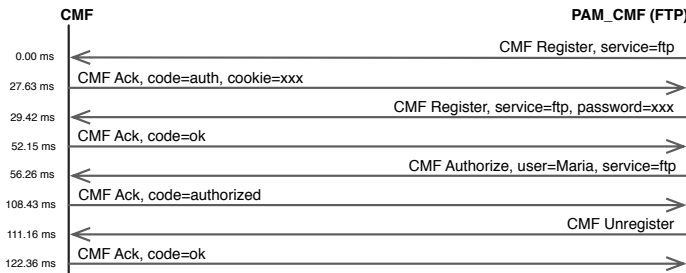
Figure 6 - Messages related to service registration and user verification, with successful authorization, captured by a monitoring application.
