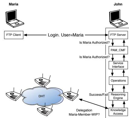
Figure 3 - Schematic of the agents and messages exchanged while authorizing an FTP session
